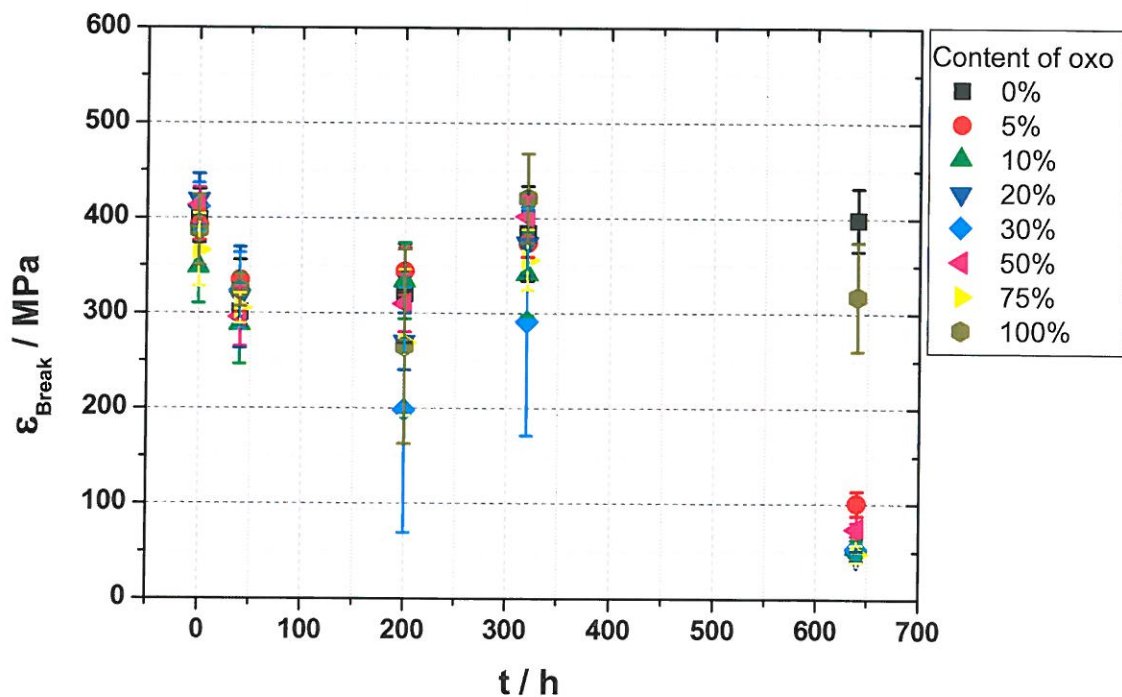
Figure 4: Breaking strain \epsilon_{Break} vs. accelerated ageing time at 70°C for LDPE films with varying content of oxo-film in LDPE-film
